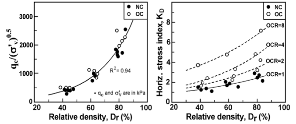
Figure 4. CPT and DMT sensitivity to stress history
