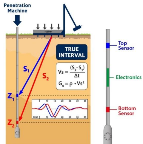
Figure 3. SDMT test layout and instrumentation
