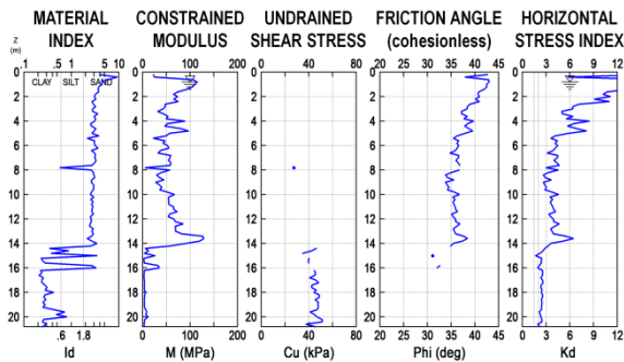
Figure 2. Example of DMT results (Fiumicino 2005)
