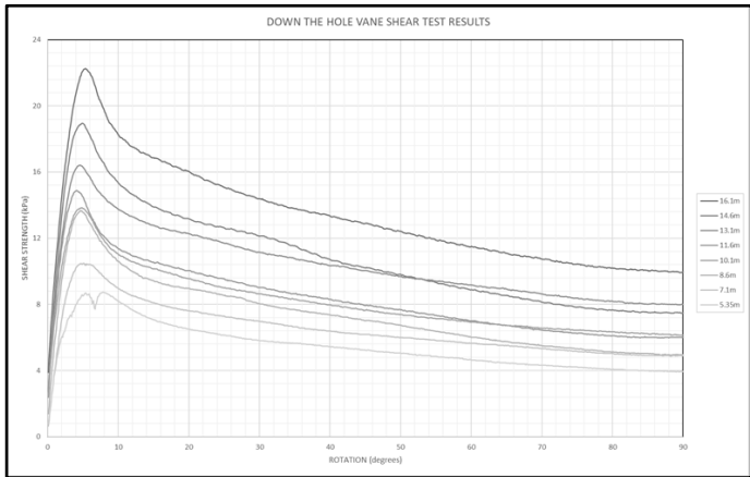
Figure 9 – Vane Shear Test Results (depth measured from seabed)
