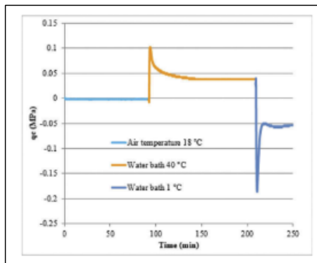
Figure 1 - Changes in zero load q_c values at varying temperatures
