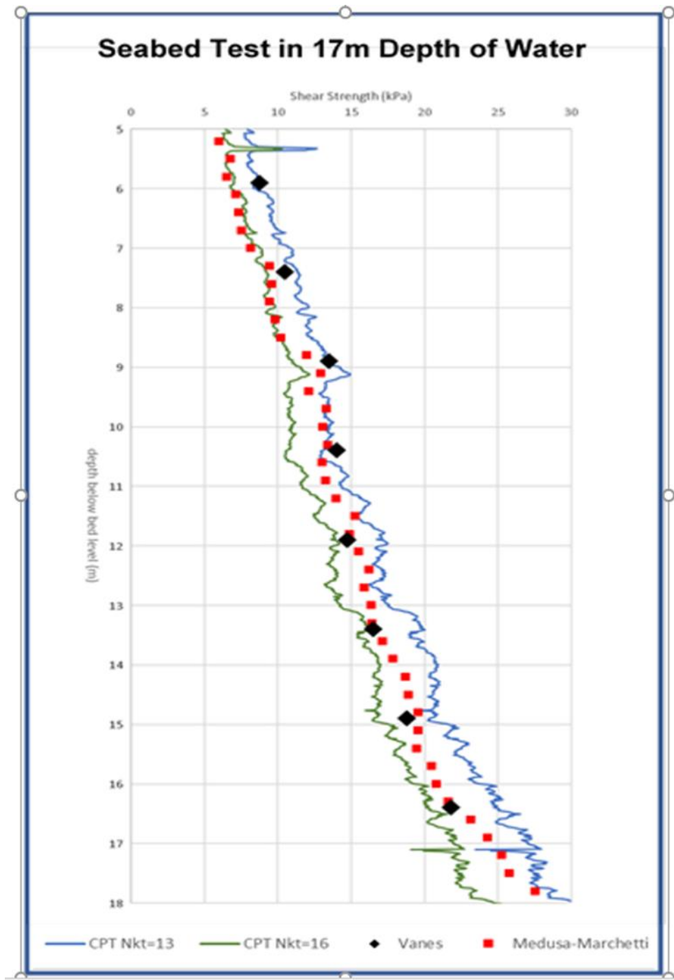
Figure 11 – All Results Plotted Together (depth measured from seabed)
