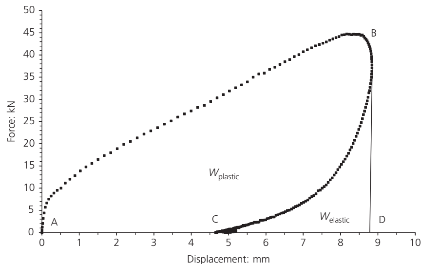
Fig. 7. Force–displacement curve for a single pass
