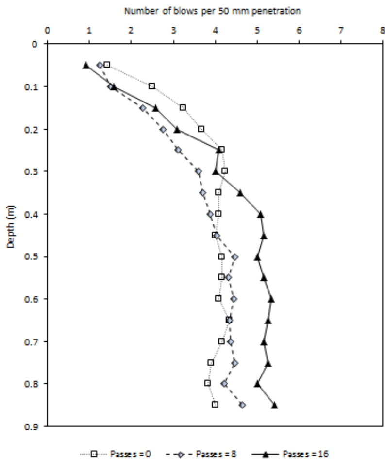
Figure 3.9: Dynamic cone penetrometer test results for 0, 8 and 16 passes
