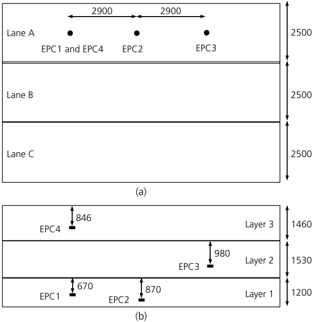
Figure 2. (a) Plan and (b) elevation views of test pad including EPC locations (all dimensions in mm)
