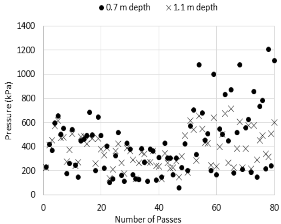
Figure 7. Measured peak pressure for each pass of the impact roller.
