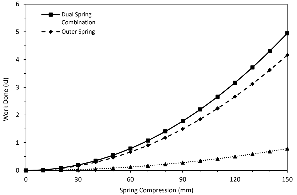
Figure 2.11: Energy contribution of the dual springs in the linkage system of the 4-sided impact roller.
