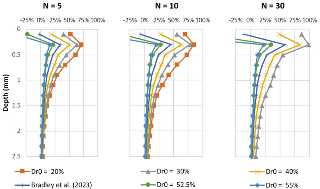
Figure 6: Distribution of average I_r with respect to Dr_0 and depth
