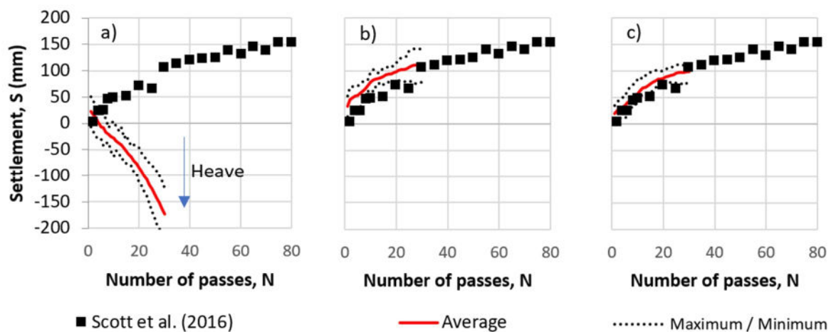
Figure 3: Surface settlement: c' = a) 1 kPa; b) 13.5 kPa; and c) 50 kPa [ 100 \text{ mm} \times 100 \text{ mm} \times 100 \text{ mm} FEs]
