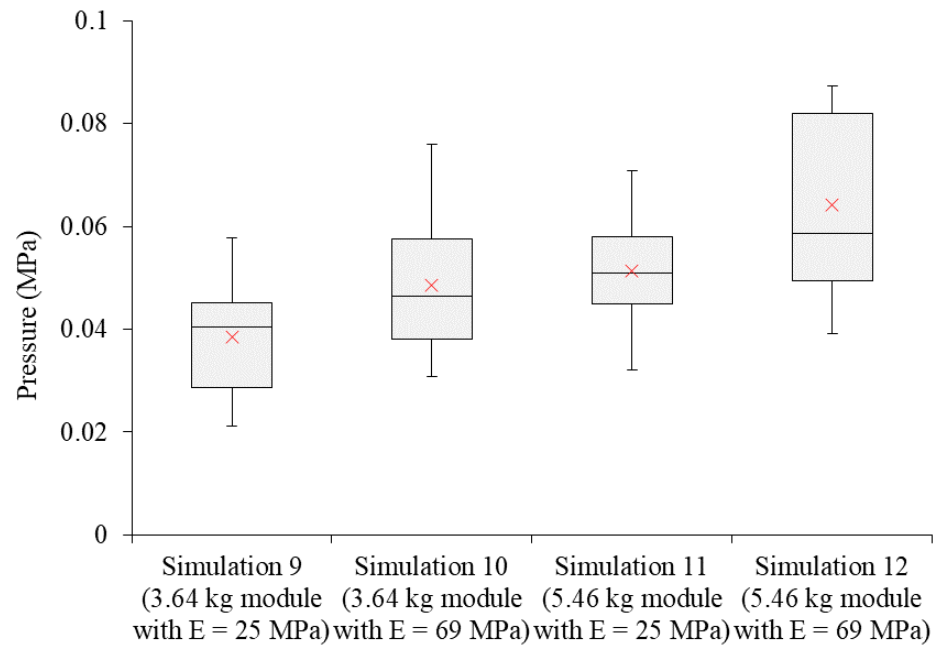
Figure 5.11: The effect of soil initial Young's modulus on the induced pressures at 55 mm depth below the ground.
