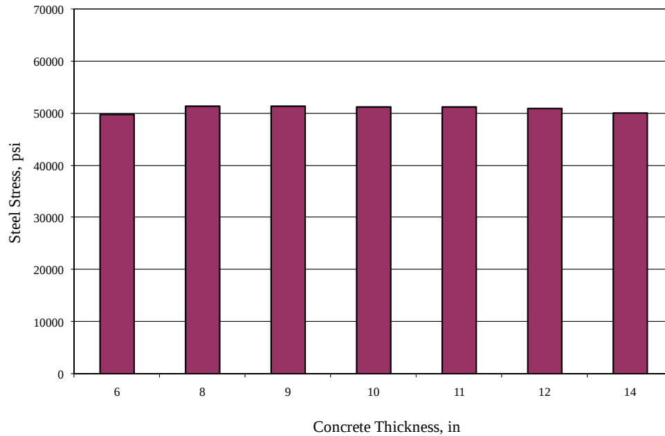
Figure 5. Effect of PCC slab thickness on steel stress (Mallela et al. 2009).
