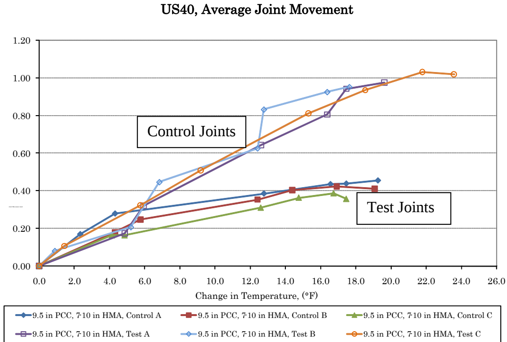
Figure 16. Joint movement at Hugo site.
