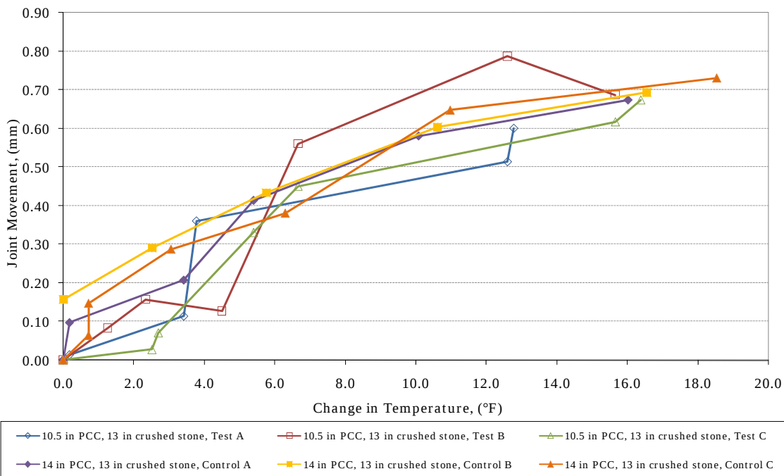
Figure 28. Joint movement at Byers site.
