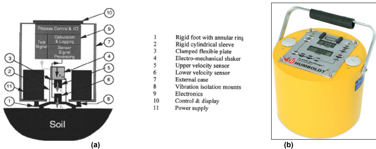
Figure 4-17 Geogauge (Soil Stiffness Gauge) Equipment – (a) Schematic cross section of instrument (from Alshibli et al., 2005); and (b) Instrument with external case housing ( www.humboldtmgf.com )
