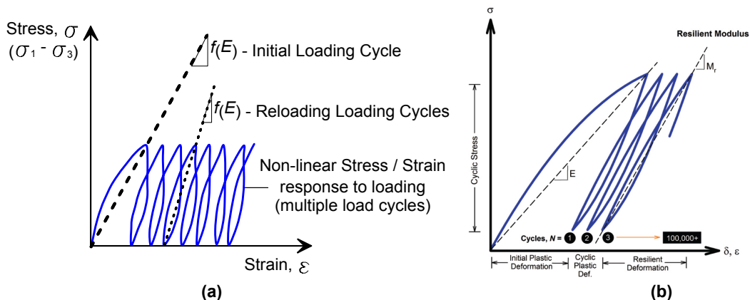
Figure 2-5 Variation in secant modulus based on cyclical loading (a) Initial Loading cycle ( E_1 ) compared to reloading cycles ( E_2, E_3 etc.), after Briaud (2001); and (b) Initial Loading cycle ( E_1 ) compared to resilient modulus ( M_R ) (from http://www.ingios.com/ )
